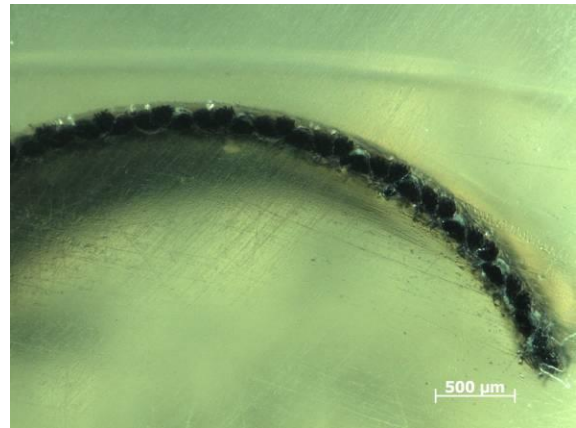
Fig. 8 Microscopic photograph Polyester with P32 PU coating
